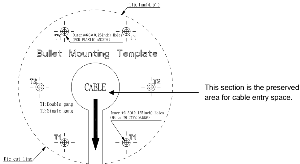
FIGURE 2 - 1: MOUNTING TEMPLATE
