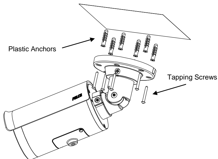
FIGURE 2 - 2: MOUNTING THE CAMERA
