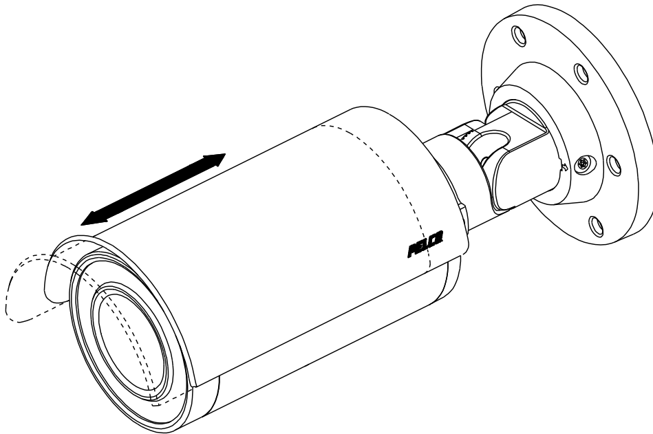
FIGURE 2 - 9: ADJUSTING THE PROTECTION SHIELD HOOD
