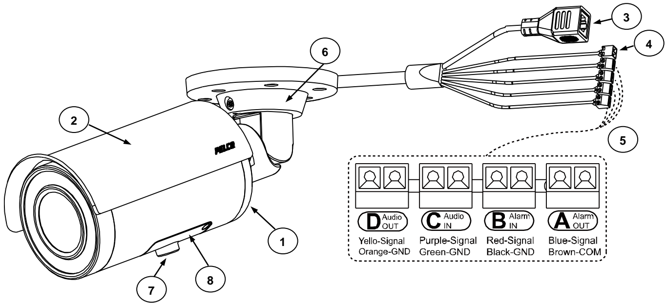
FIGURE 1-2: CAMERA CONNECTIONS AND FEATURES 1/2
