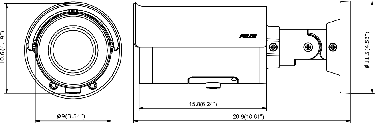
ENVIRONMENTAL IR BULLET
