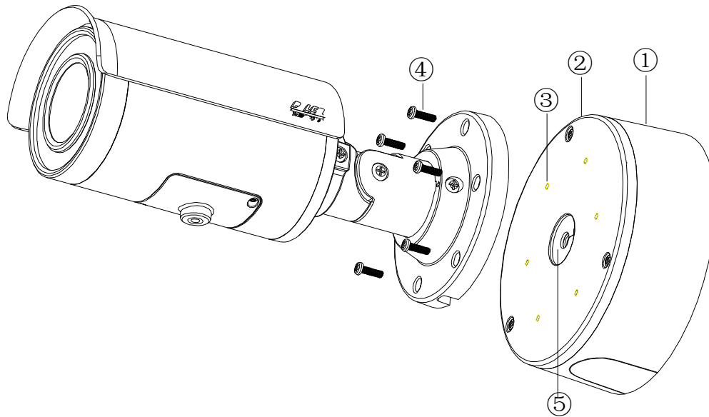
FIGURE 2-5: SURFACE MOUNT WITH IBP2BBAP-ES
