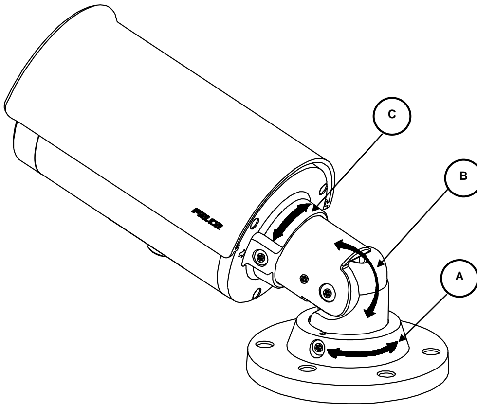
FIGURE 2 - 8: ADJUSTING THE CAMERA POSITION
