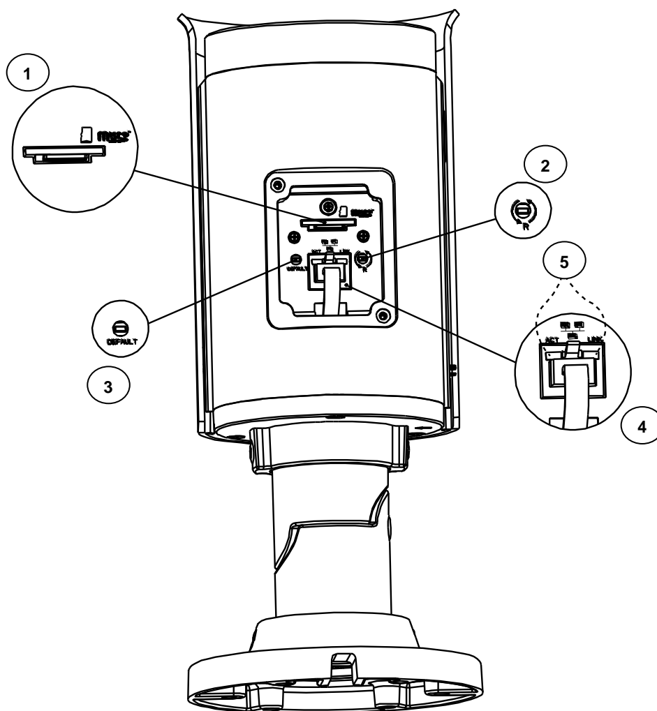
FIGURE 1-3: CAMERA CONNECTIONS AND FEATURES 2/2
