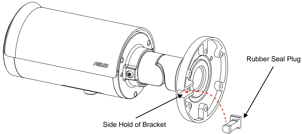
FIGURE 2 - 7: RUBBER SEAL PLUG APPLYING
