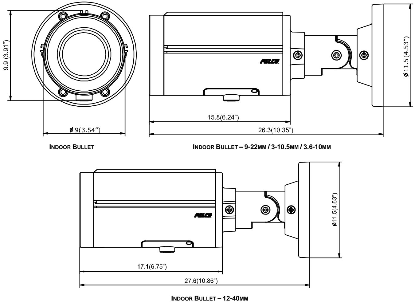
FIGURE 1-1: PHYSICAL DIMENSIONS
