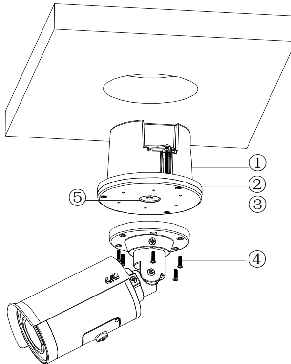
FIGURE 2-6: IN-CEILING INSTALLATION WITH IBP2BBAP-EI
