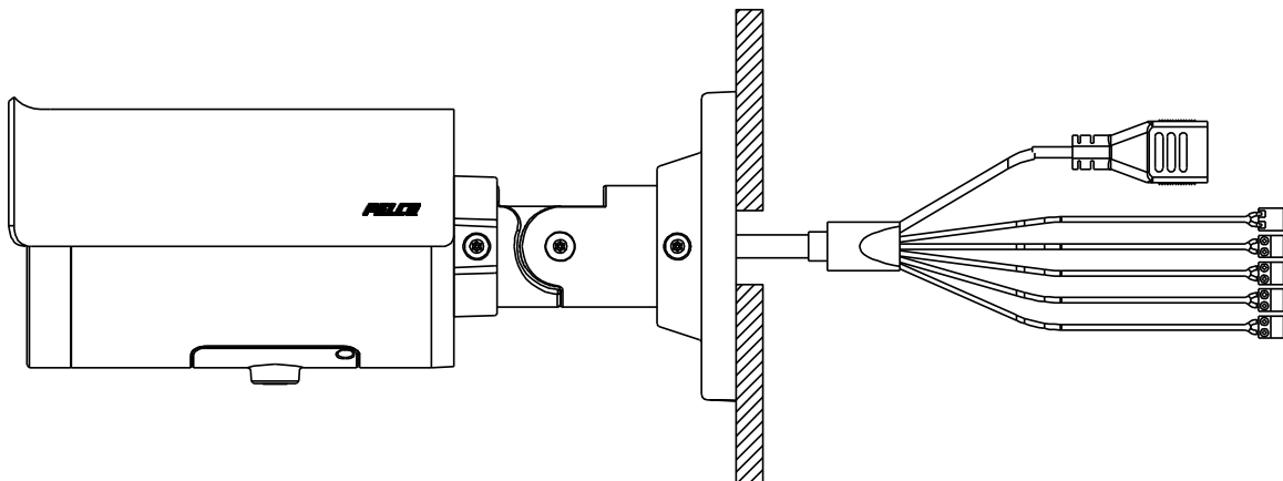
FIGURE 2 - 4: CONNECTING THE WIRES TYPE II – MOUNTING SURFACE HOLE
